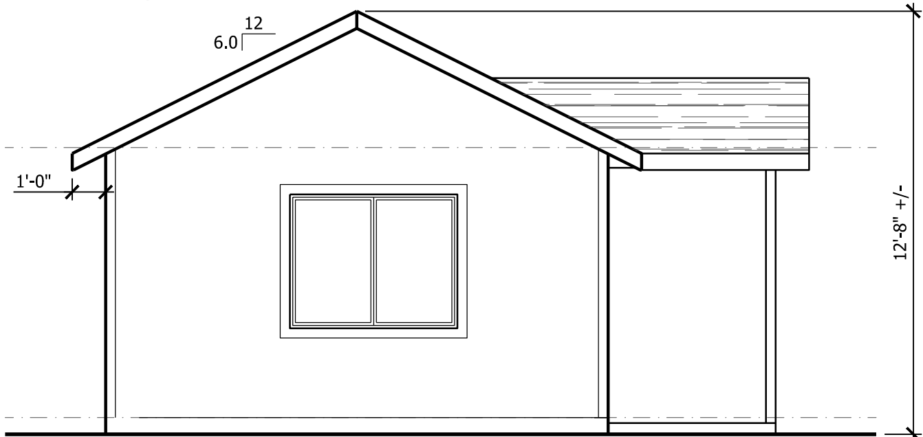
D LEFT ELEVATION
