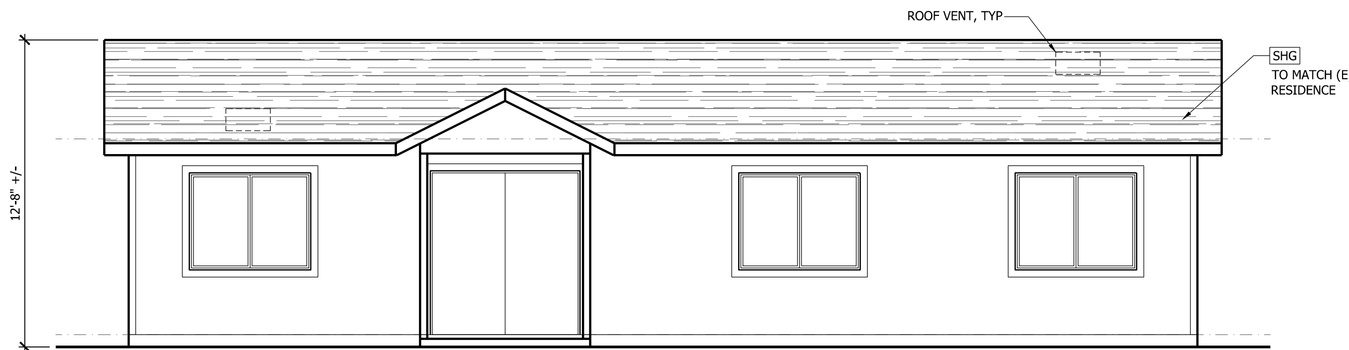
A FRONT ELEVATION
