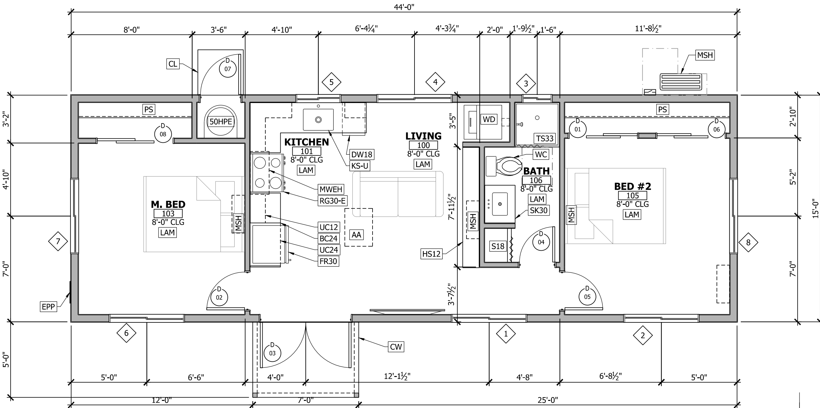
1 FLOOR PLAN
